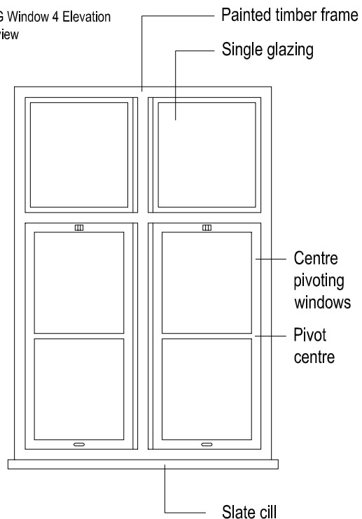
PROPOSED Window 4 Elevation Internal view 1:20
