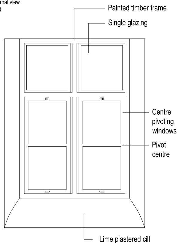
PROPOSED Window 5 Elevation Internal view 1:20
